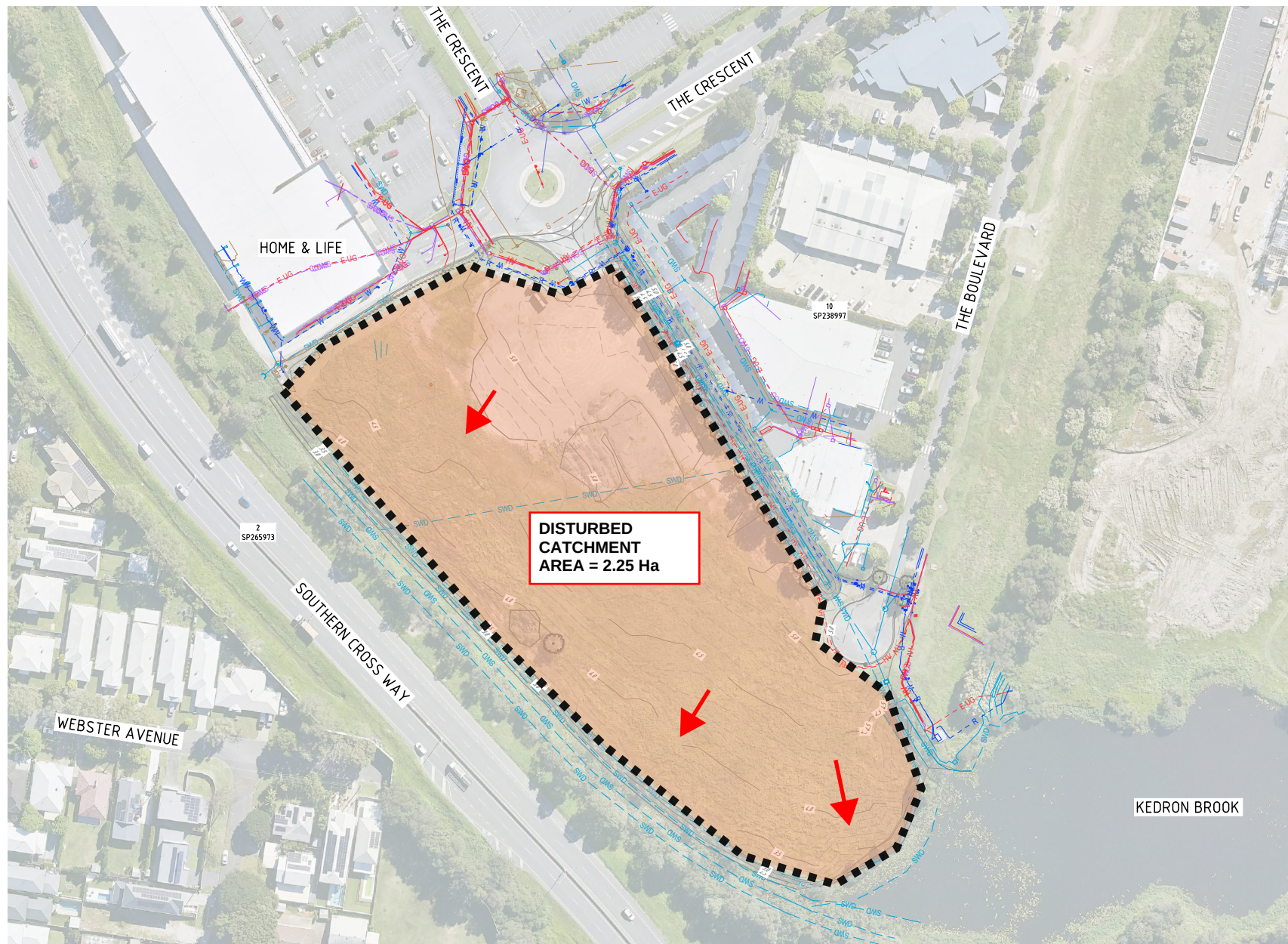
DISTURBED CATCHMENT LAYOUT PLAN
